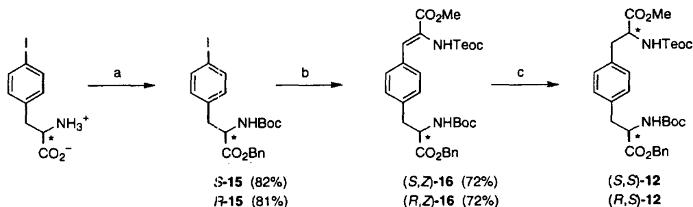
Scheme 2. (a) 1. (Boc) 2 O, K 2 CO 3 , dioxane:H 2 O 1:1; 2. BnBr, DMF; (b) 2 , Pd(OAc) 2 , NaHCO 3 , Bu 4 NCl, DMF, 85–90°C, 18 h; (c) H 2 , [Rh(COD)(( R,R )-DIPAMP)] + BF 4 − , MeOH
