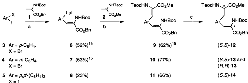
Scheme 1. (a) \text{Pd}(\text{OAc})_2 , \text{NaHCO}_3 , \text{Bu}_4\text{NCl} , DMF, 85\text{--}90^\circ\text{C} , 18 h; (b) \text{Pd}(\text{OAc})_2 , \text{NaHCO}_3 , \text{Bu}_4\text{NCl} , DMF, 85\text{--}90^\circ\text{C} , 18 h; (c) \text{H}_2 , [\text{Rh}(\text{COD})(\text{bisphosphine})]^+ \text{X}^- , MeOH. List of abbreviations: Bn=benzyl, Boc= tert -butoxycarbonyl, Cbz=benzyloxycarbonyl, COD=1,5-cyclooctadiene, dppe=1,2-bis(diphenylphosphino)ethane, Teoc=2-(trimethylsilyl)ethyloxycarbonyl
